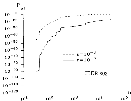
Fig. 2. P_{ue}(n) versus n for the IEEE-802 code on the BSC's with \epsilon = 10^{-3} and 10^{-6} .
